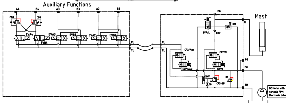
HYDRAULIC SCHEMATIC
