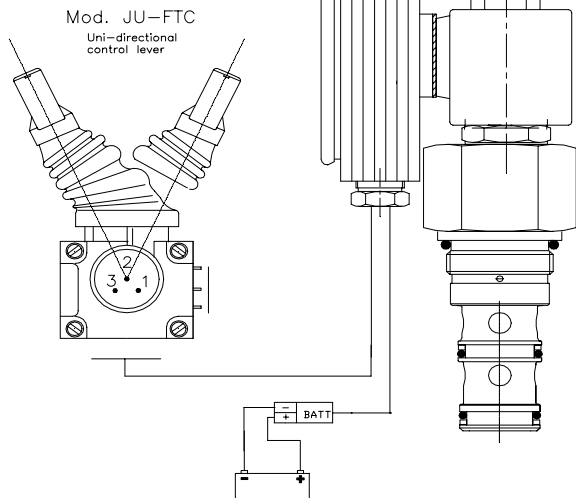
Mod. FP-REC-47 Proportional Flow Regulator
